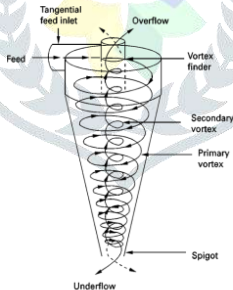
Fig 5. Schematic diagram of a hydrocyclone
