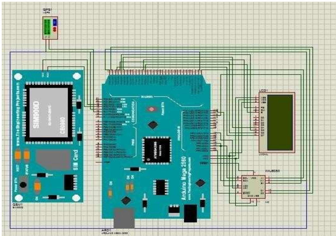
Fig -3: Circuit Diagram
