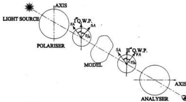
Fig. 1 Arrangement for circular polariscope
