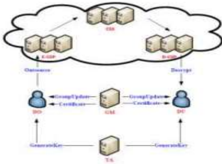
Figure 1: System Architecture
