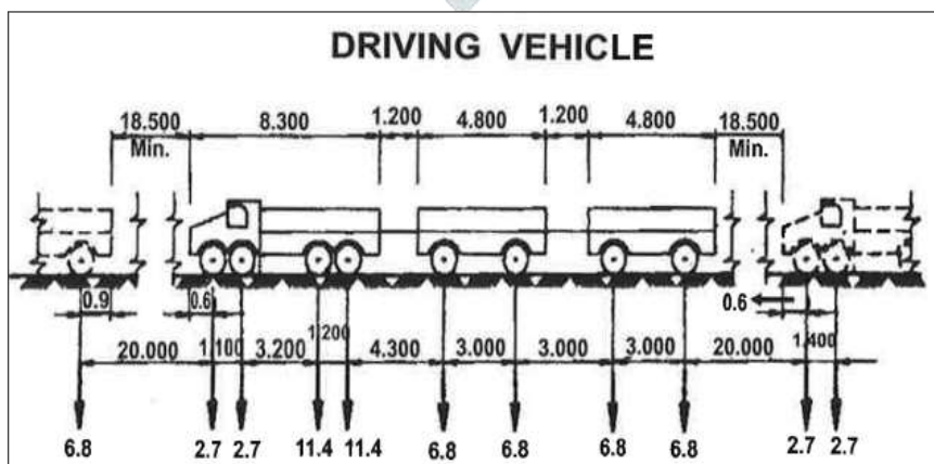
FIG2. CLASS A WHEELED LOAD
