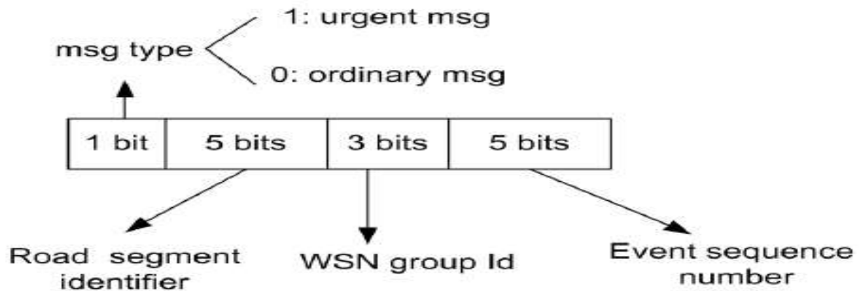
Figure-8: forewarning information's header added by the WSN-Gateway
