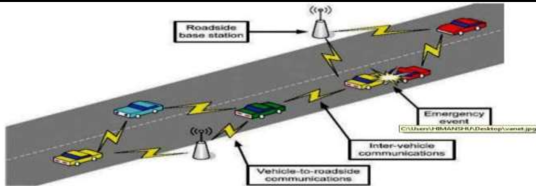
Figure-1: VANET
