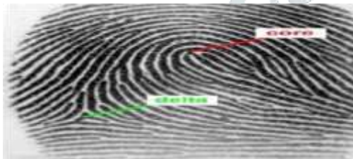
Fig 13. Fingerprint detection
