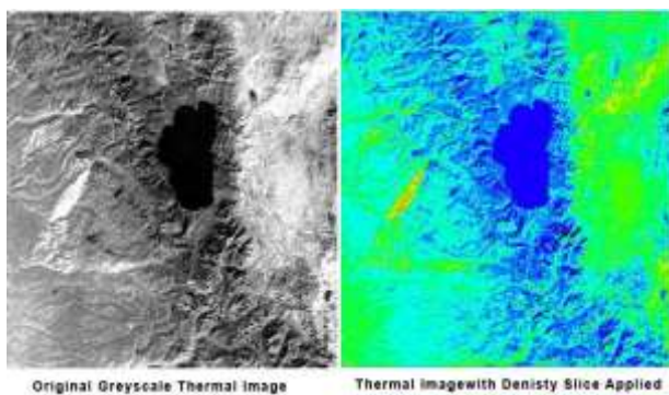
Fig4. Density slicing
