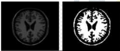
Fig9. Thresholding Segmentation
