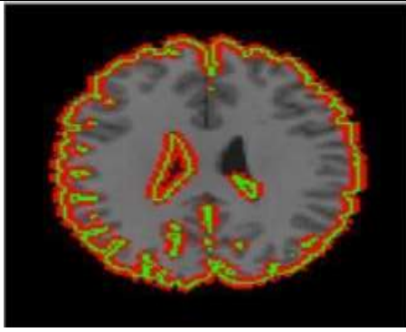
Fig 8. Region-Based Segmentation
