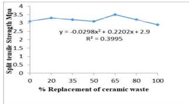
Fig. 4. Representation of Split tensile Strength reported by Anderson et.al [14]
