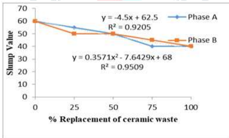
Fig.1. Representation of slump value reported by Tavakoli et al.
