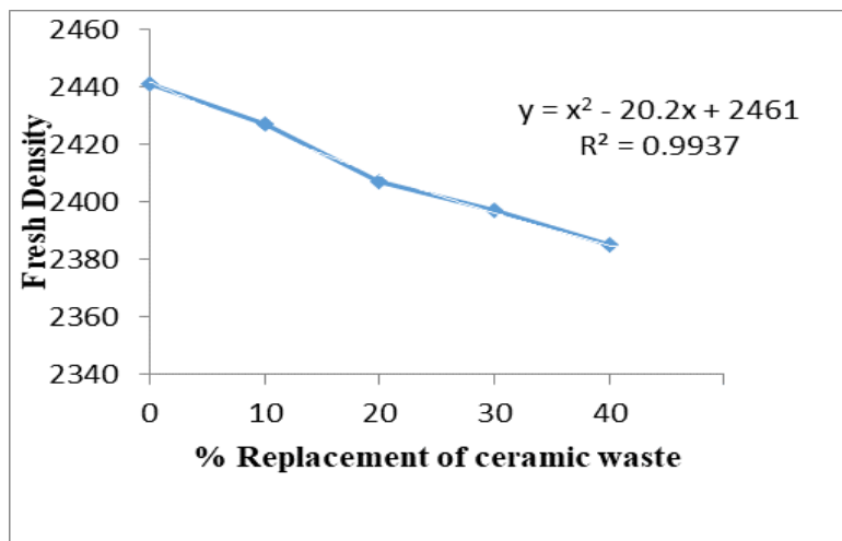
Fig.2. Representation of fresh concrete density reported by Tavakoli et al. [13]
