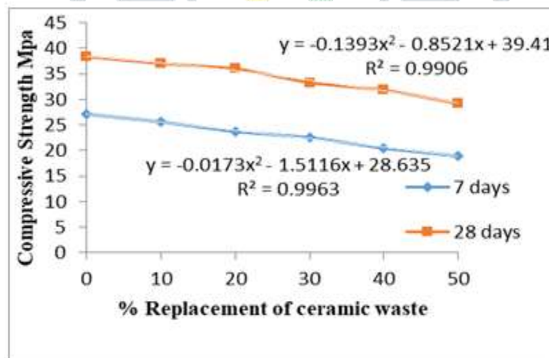
Fig. 3. Representation of Compressive Strength reported by Raval et al. [12]
