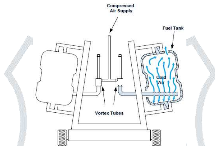
Fig. 3 Cooling Blow Molded Fuel Tanks.
