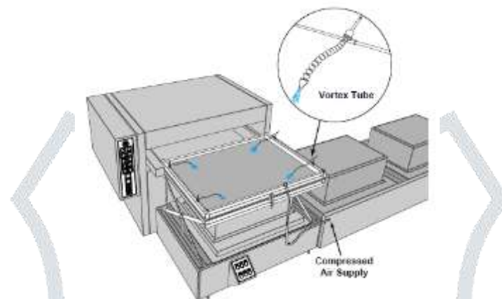
Fig. 5 Cooling Vacuum Formed Parts
