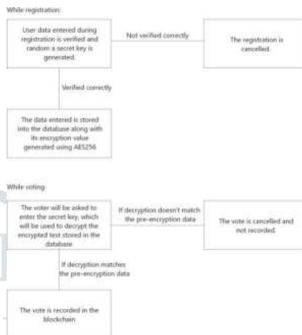
fig1. Flowchart for identity verification
