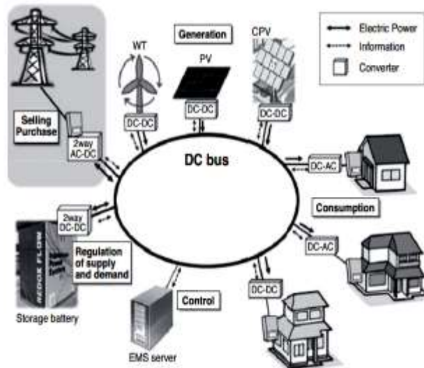
Figure 1: Microgrid Component
