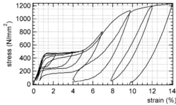
Figure 1 Stress-strain relation of SMA wire under room temperature 16 degree centigradestress strain property of SMA bars
