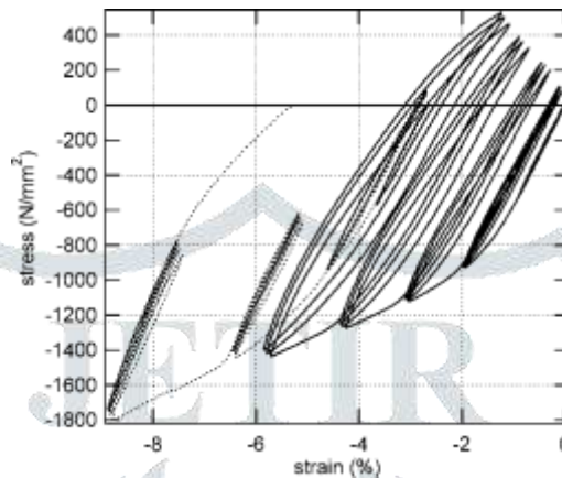
FIGURE 3 STRESS-STRAIN RELATION FOR STATIC COMPRESSION TEST
