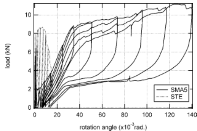
Figure 12 Load vs. rotation angle of the beams
