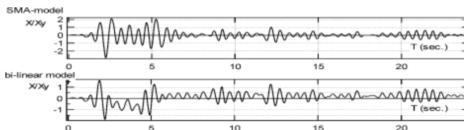
Figure 10 Time history of Response of SMA-model & bi-linear model
