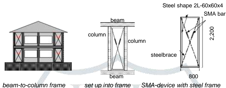
FIGURE 8 SMA DEVICE AND ITS SET UP INTO A BEAM-TO-COLUMN FRAME
