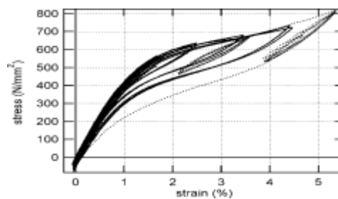
FIGURE 2 STRESS-STRAIN RELATIONS FOR STATIC TENSION TEST
