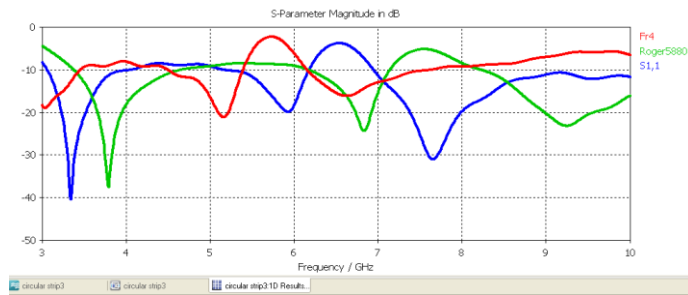
Figure 4: Effect of substrate material on the antenna performance
