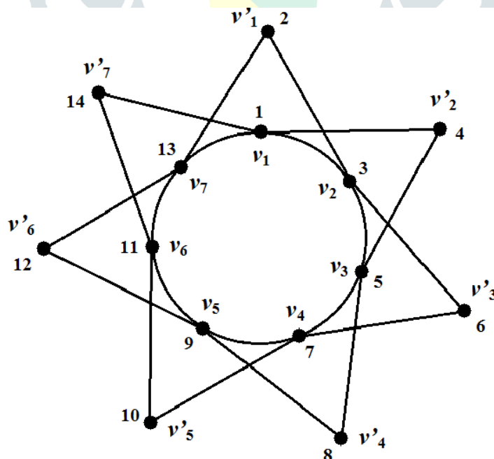
Figure 2. Labeling the vertices of Spl(C7) Checking the relative prime of each pair of vertices v_i and v_{i+1} which are not relatively prime. We get the following graph. v_i and v_{i+1} and mark the vertex v_i and v_{i+1} within circles
