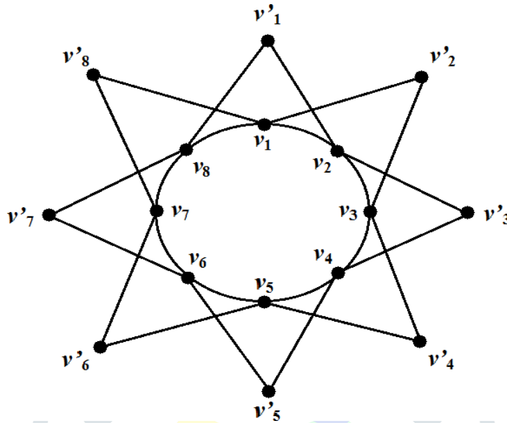
Figure 5. Split graph of C8, Spl(C8)
