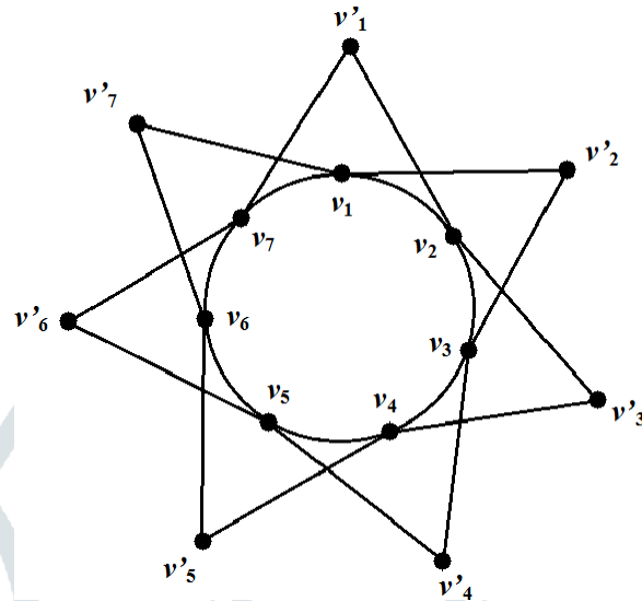
Illustrations 1- Let n = 7 ( n is odd), Spl(C7) is a prime graph
