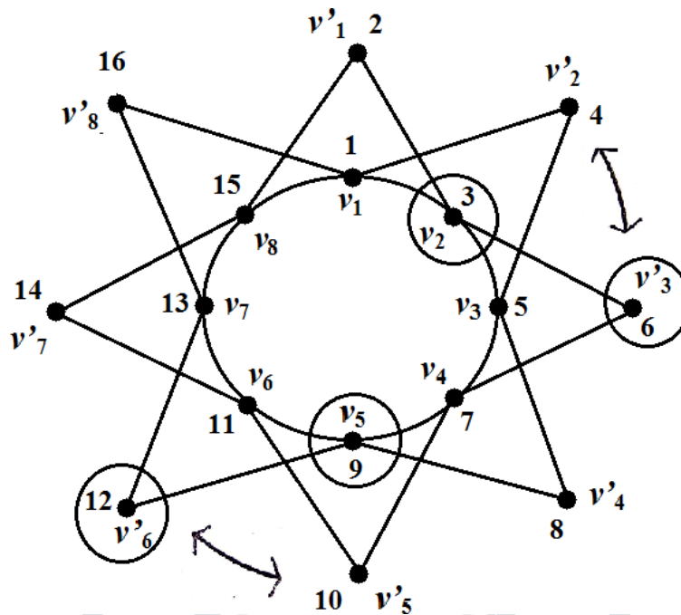
Figure 7. Checking and Encircling the non – prime pairs
