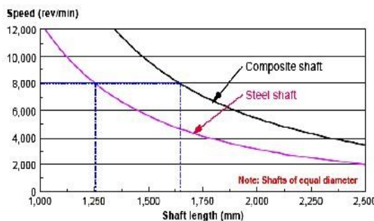
Fig.3. The effect of shaft length on critical speed
