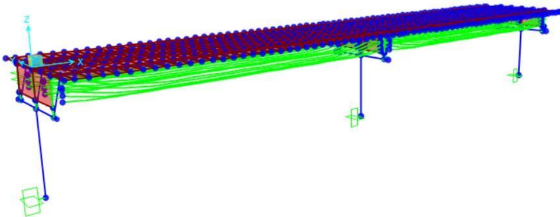
Fig 8 3D MODEL
