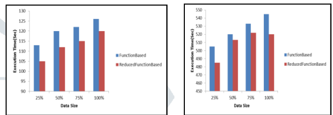
Fig. 1 Execution time on the WorldCup98 dataset under different data sizes for querytype1 and querytype2.
