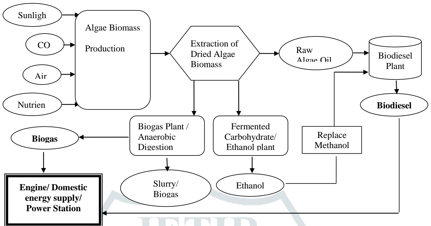
Fig. 1. A Model for Integrated Energy Generation from Microalgae
