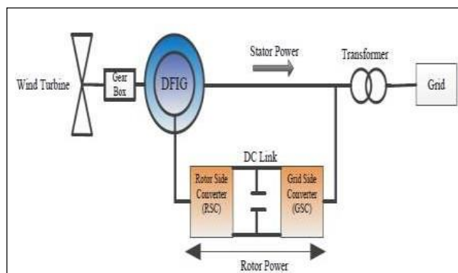
Fig. 1: DFIG based Wind Turbine System
