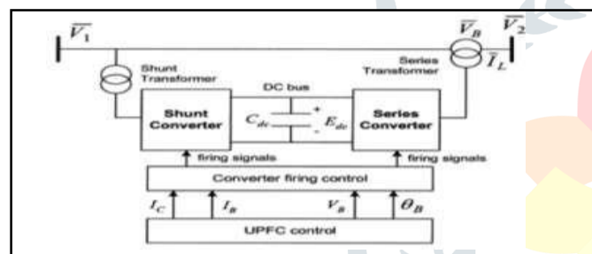
Fig. 2: Unified Power Flow Controller
