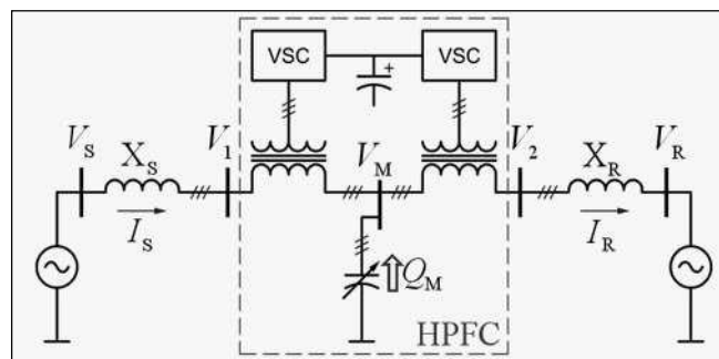
Fig. 3: Hybrid Power Flow Controller
