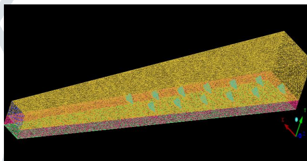
Fig. 6 meshing for ribbed divergent duct with staggered arrangement
