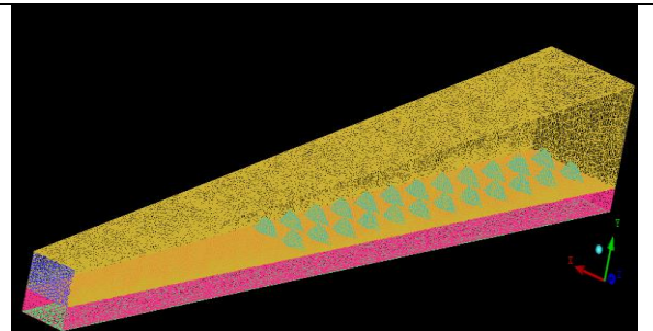
Fig.5 meshing for ribbed divergent duct with inline
