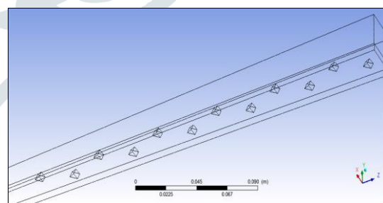
Fig. 2.c. divergent ribbed duct with staggered
