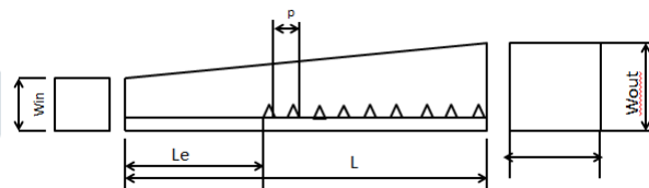
Fig.2 Test Geometry
