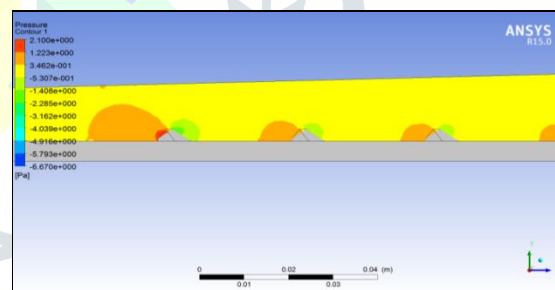
Fig. 9 pressure contour for ribbed divergent duct
