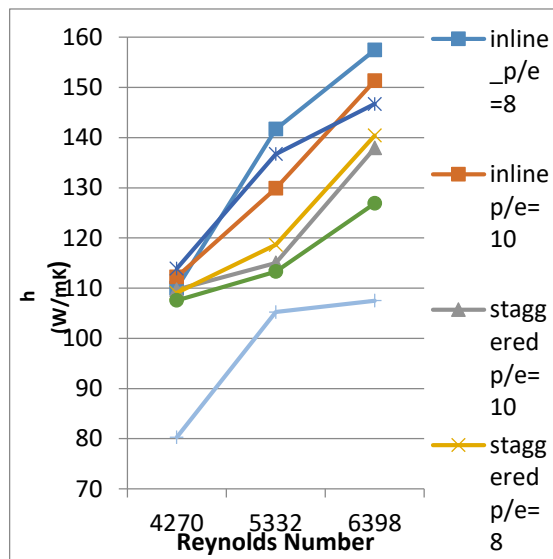
Fig. 11 Variation of heat transfer coefficient with Re
