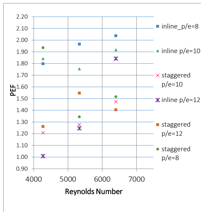
Fig. 14 Performance enhancement factor
