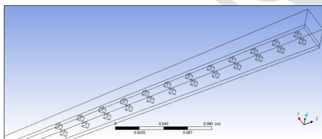
Fig. 2.b. Divergent duct with ribs inline arrangement
