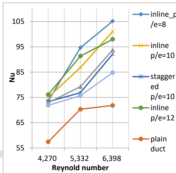
Fig. 12 Variation of Nusselt Number with Re
