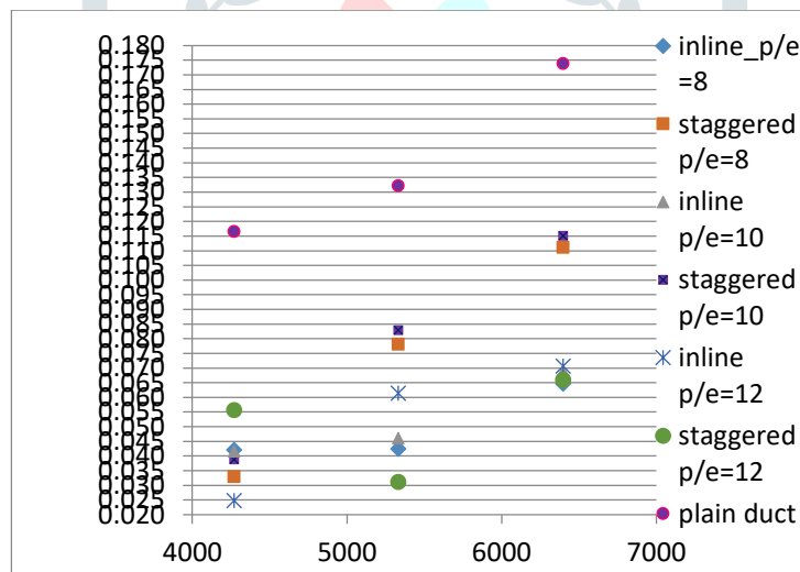
Fig. 13 Friction factor Vs Re
