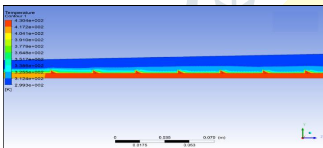
Fig. 8 Temperature Contour for ribbed divergent duct
