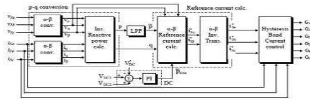
Fig -3 Block diagram of shunt APF control
