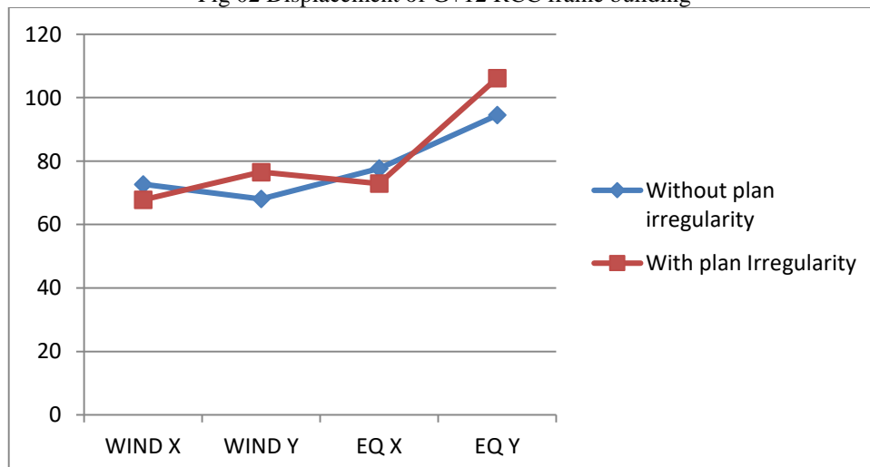
Fig 03 Displacement of G+15 RCC frame building
