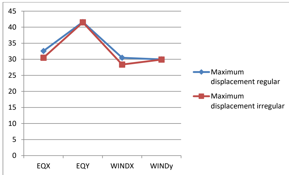
Fig 01 Displacement of G+7 RCC frame building
