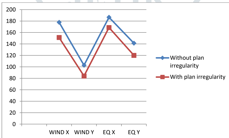
Fig 05 Story moment of G+12 RCC frame building
