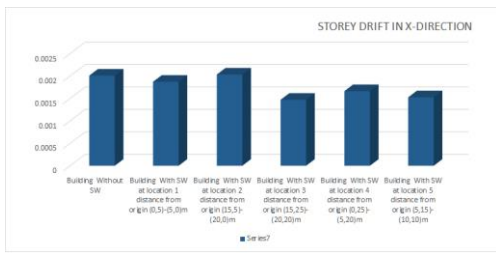
Static Storey Drift in X-Direction (Unitless)
