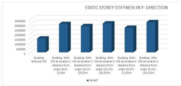
Static Storey Stiffness in Y-Direction (KN/M)
