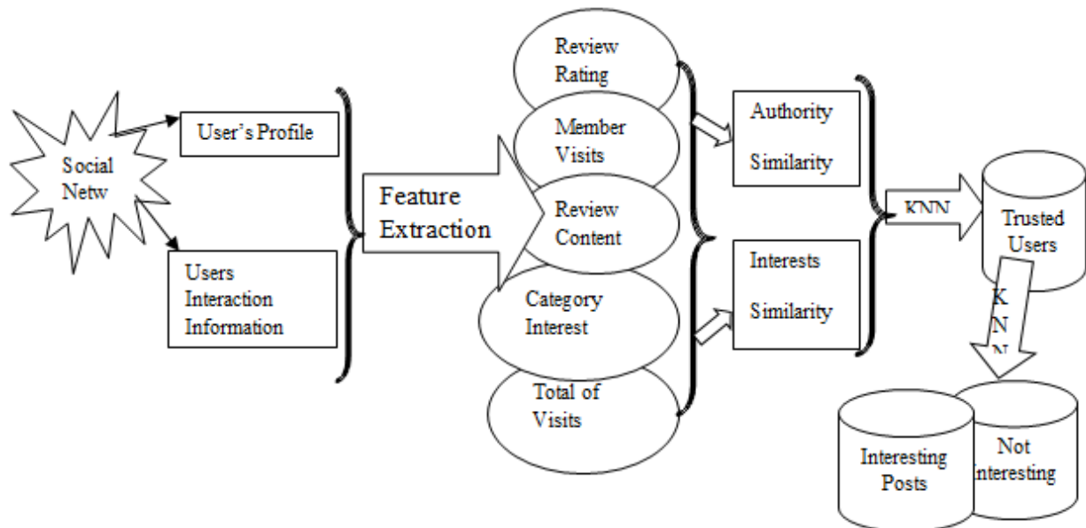
Fig.1. Model for Predicting Interesting Posts from Trusted Users
