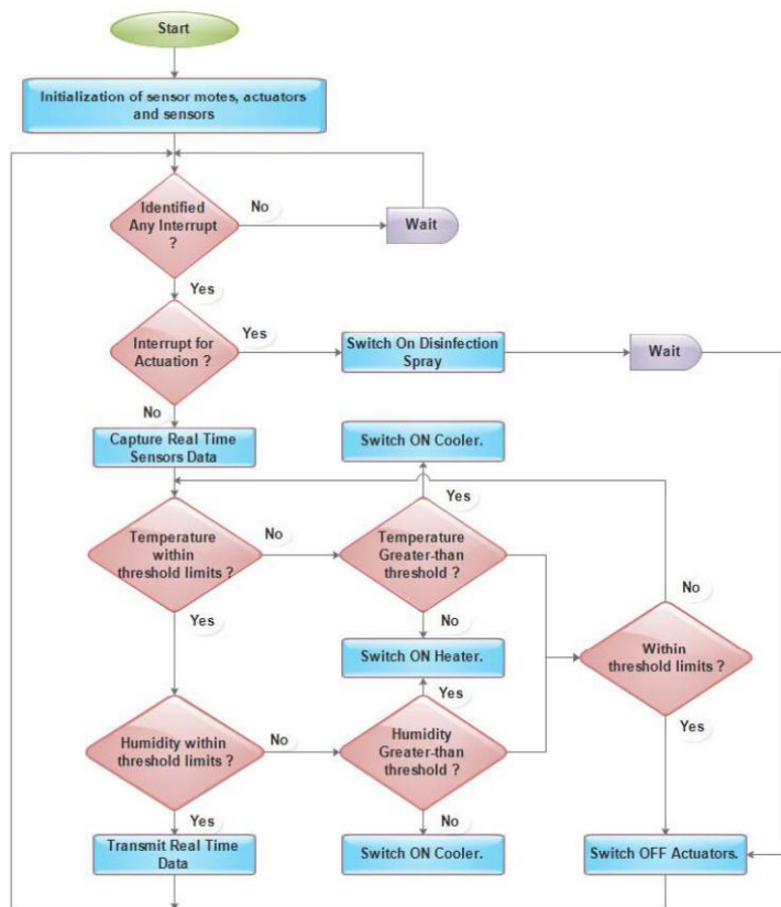
Flow chart for actuation system
