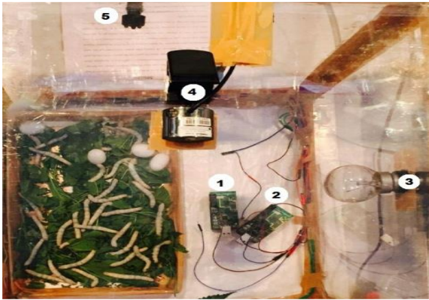
Top View of Monitoring and Actuation system for sericulture.
