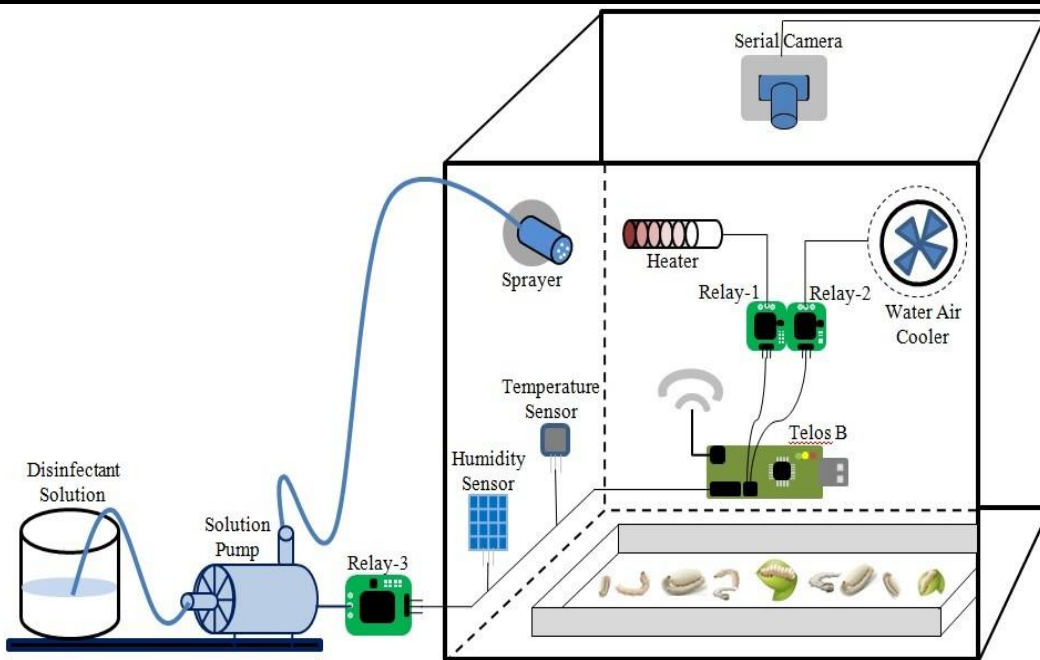
IoT based Block Representation of the Sericulture Monitoring and Actuation System
