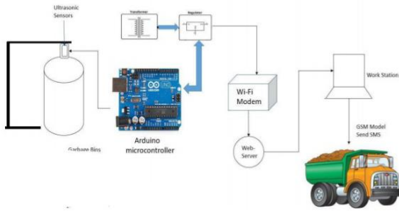
Figure 4. Hardware components connection.[6]
