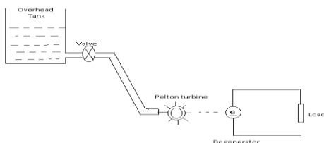
Fig (a) micro hydro plan Potential energy of water
