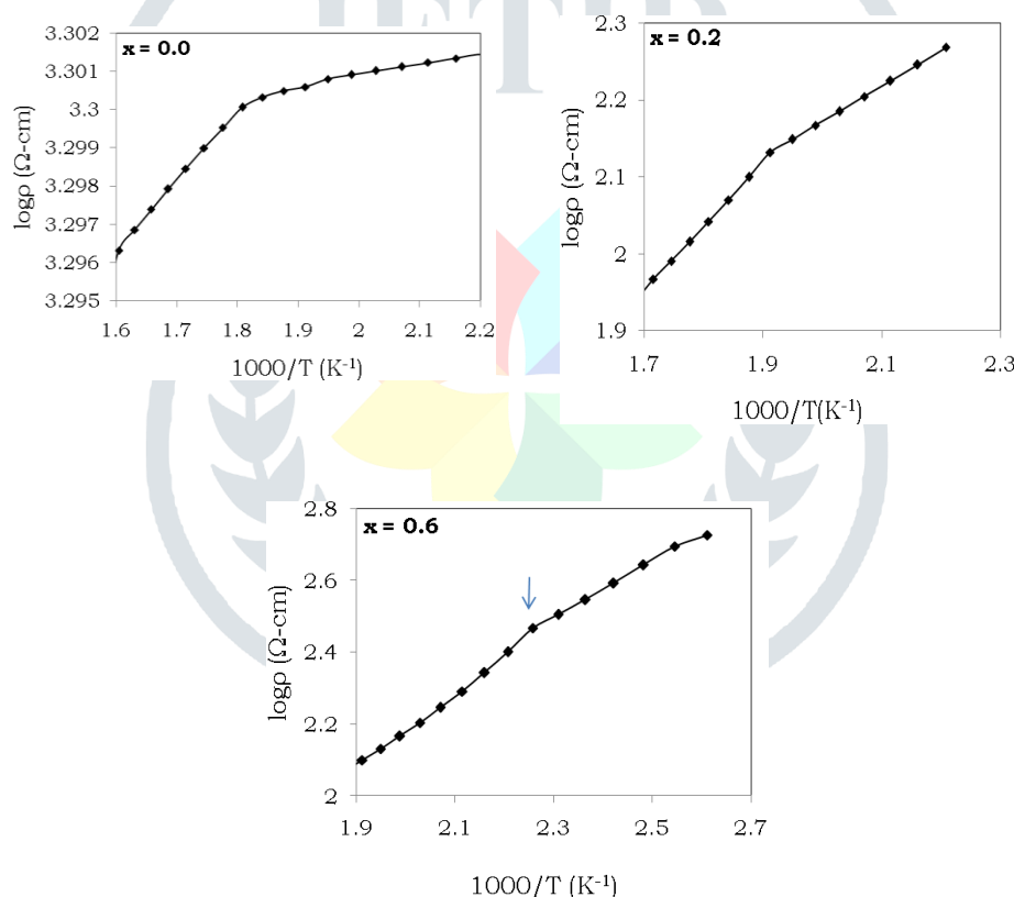
Fig. 2 : Variation of \log \rho versus 1000/T of \text{Y}_3\text{In}_x\text{Fe}_{5-x}\text{O}_{12} . ( x = 0.0, 0.2 and 0.6 ).
