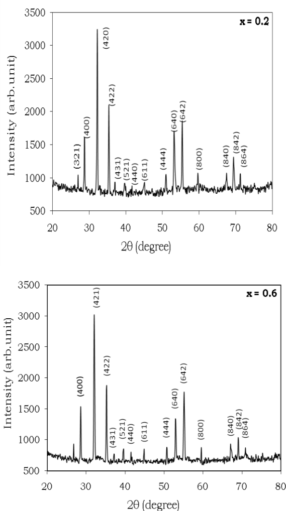
Fig. 1(a): Typical XRD patterns of Y_3In_xFe_{5-x}O_{12} . ( x = 0.2 and 0.6 )
