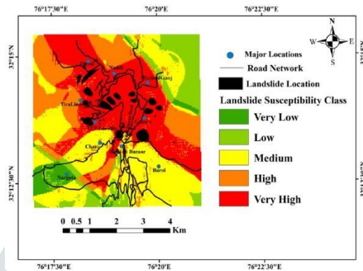
Fig.5 Landslide susceptibility zonation map of Dharamshala.
