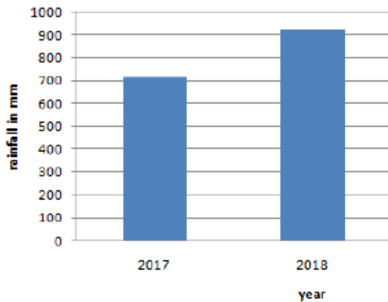
Fig.4 showing monsoon rainfall intensity graph from 2017 to 2018
