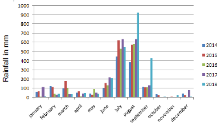
Fig.2 Kangra, H.P rainfall data from 2014 to 2018
