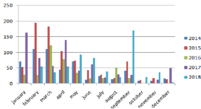
Fig.3 rainfall data of Lahul and spiti 2014-2018
