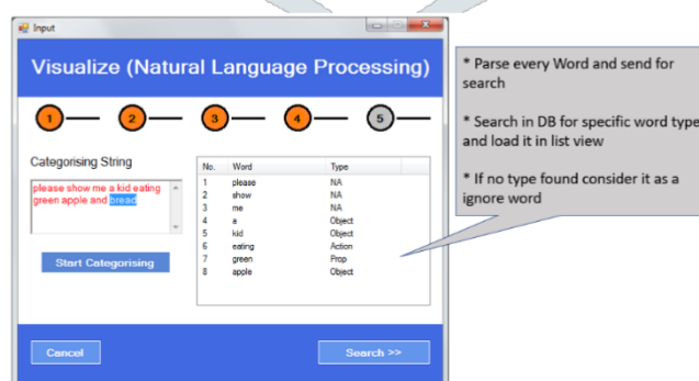
Figure 6. Categorization of words
