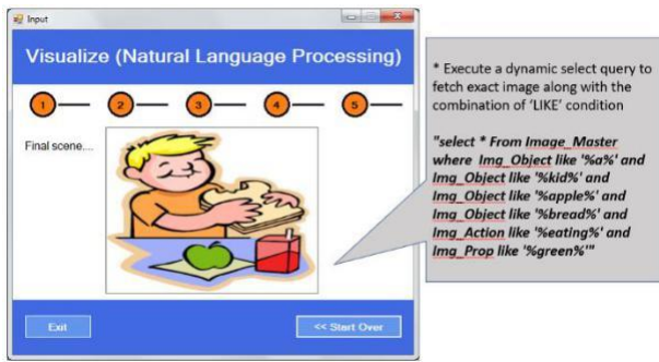
Figure 7. SQL query based search
