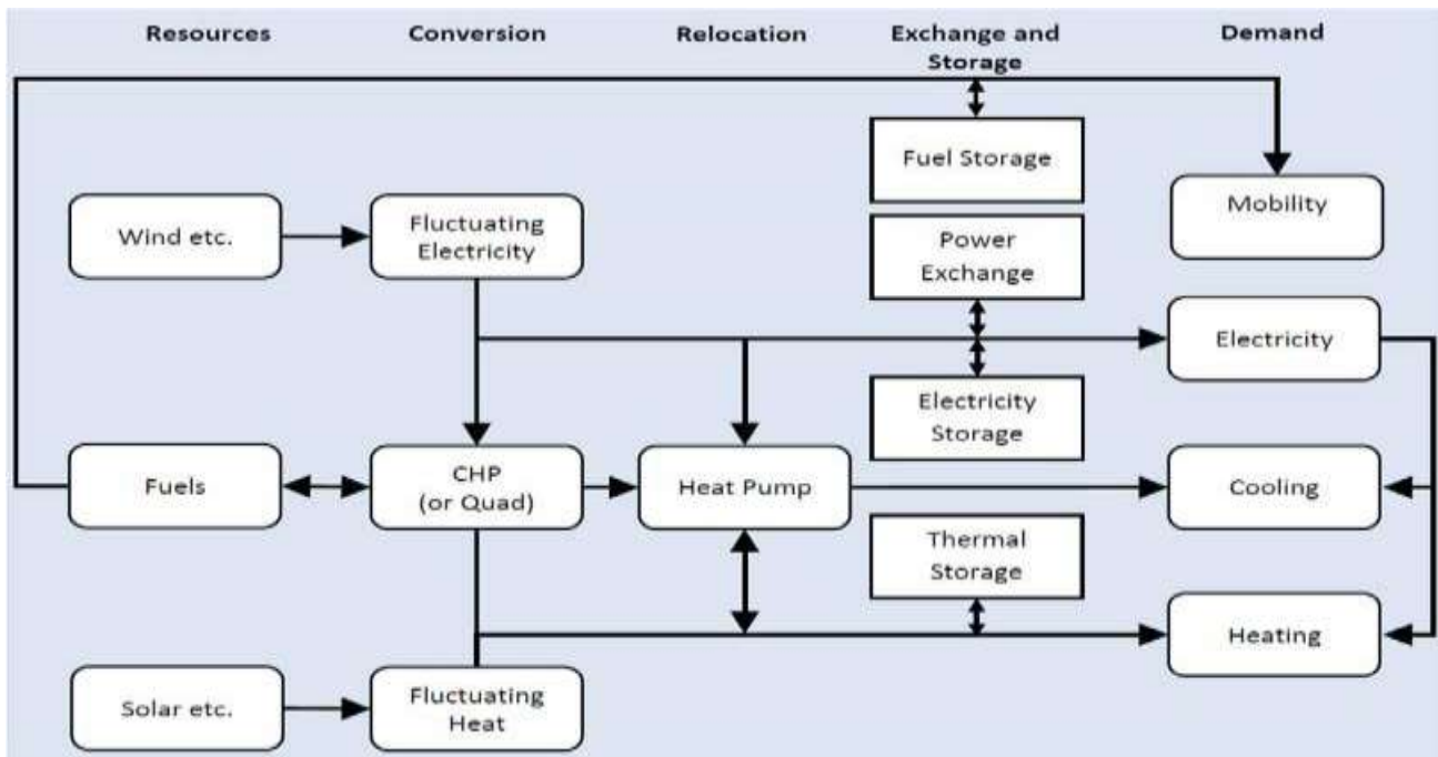
Figure: Illustration of a Smart Energy System based on the integration of the power, heating, cooling, gas and transportation sectors and infrastructures.
