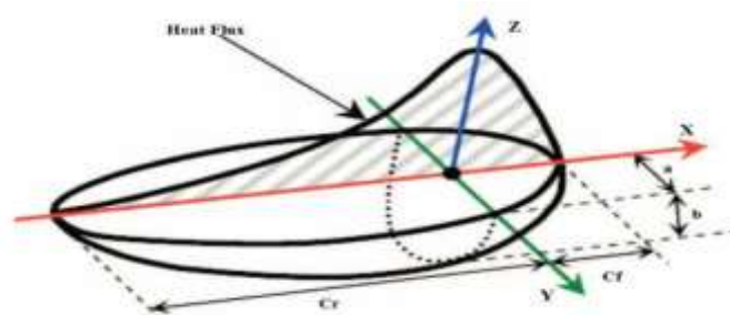
Fig 1. Double ellipsoidal heat source [7]
