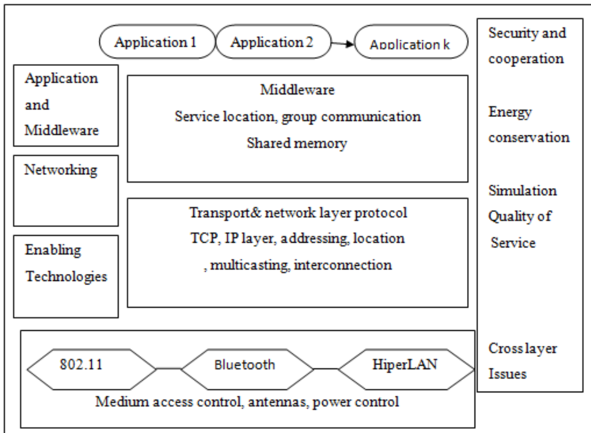
Figure 6 MANET Architecture
