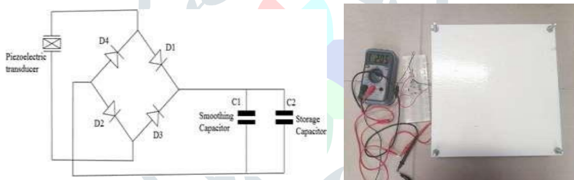
Figure 1. Diagram of the full-wave bridge rectifier with smoothing and storage capacitor
