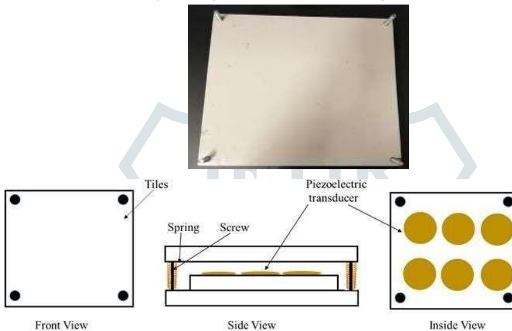
Figure 10. Model of piezoelectric tile with 6 cell of piezoelectric tile
