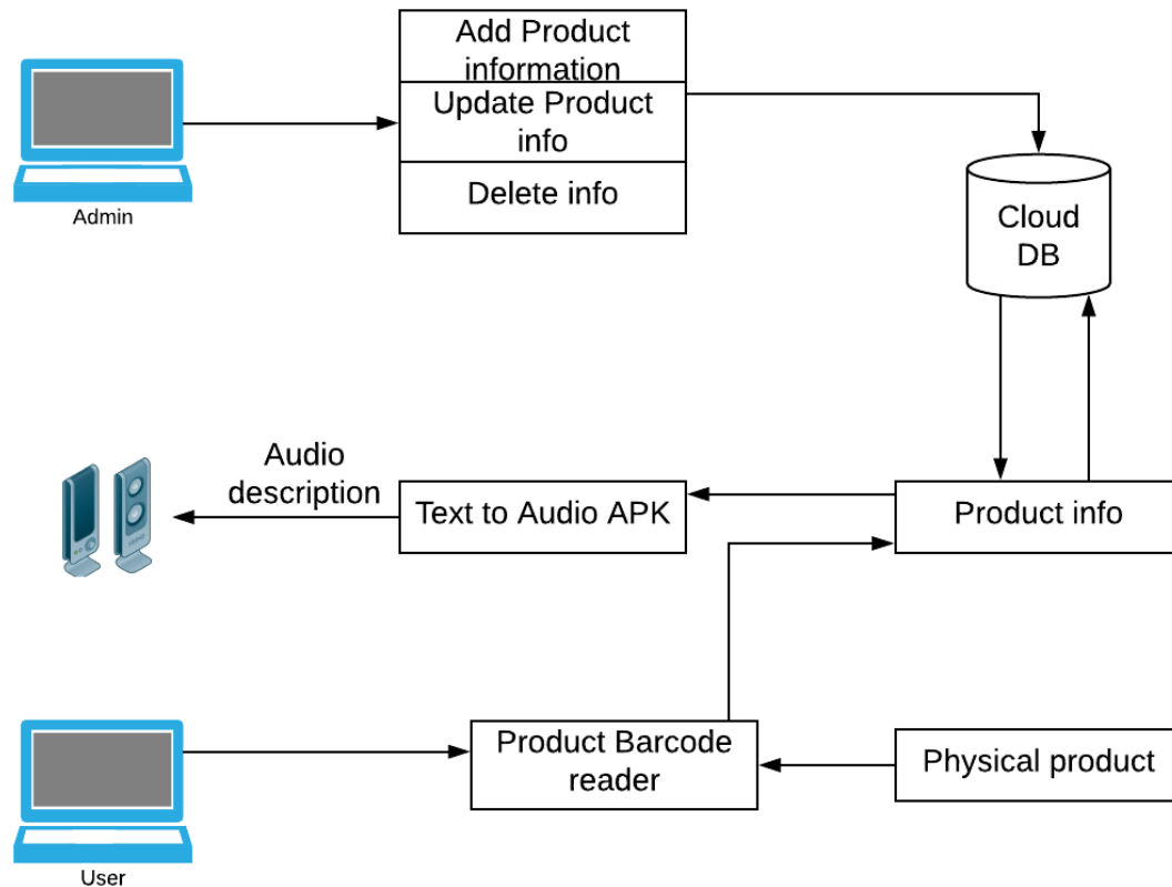
Figure 1 : System Architecture
