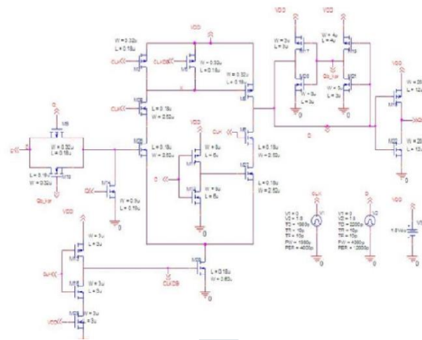
Spice capture of CDMFF
