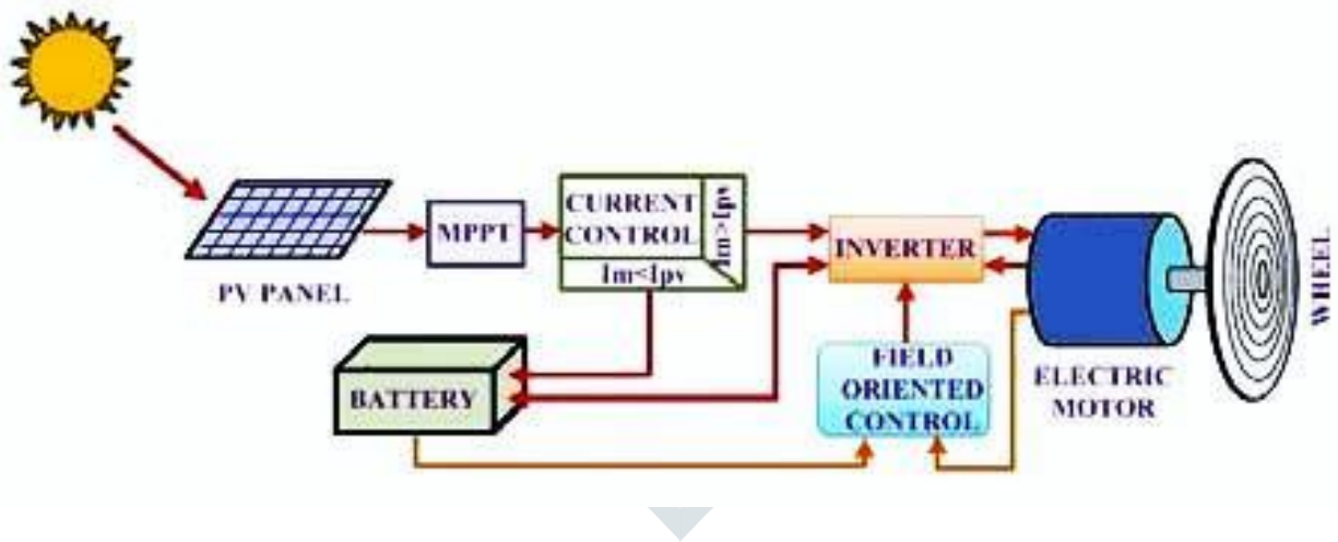
FIGURE 2: THE BLOCK DIAGRAM OF SOLAR ELECTRIC VEHICLE.
