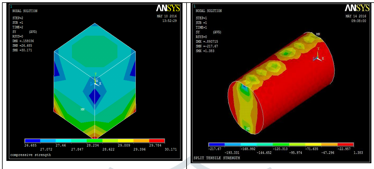
Figure 3: Stress variation for cube and cylinder specimens
