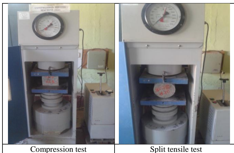
Figure 2: Testing of specimens
