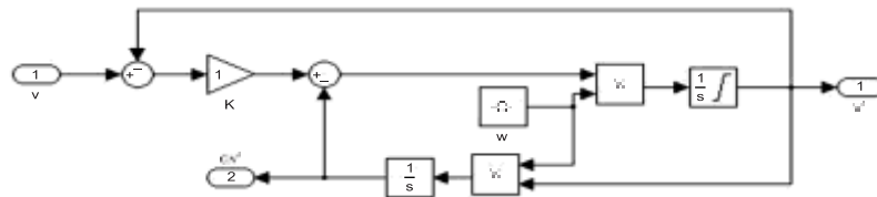
Figure 2: SOGI Quadrature signal generator
