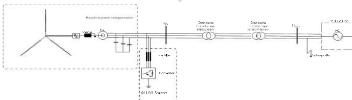
Figure 1: FSIG wind farm integration with STATCOM
