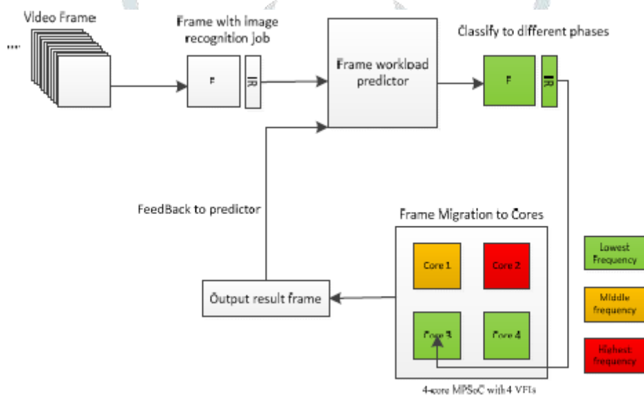
Fig. 2. DVFS based parallel scheduling [4].
