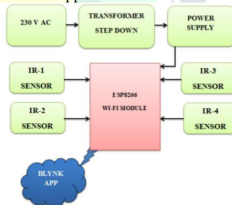
Block diagram
