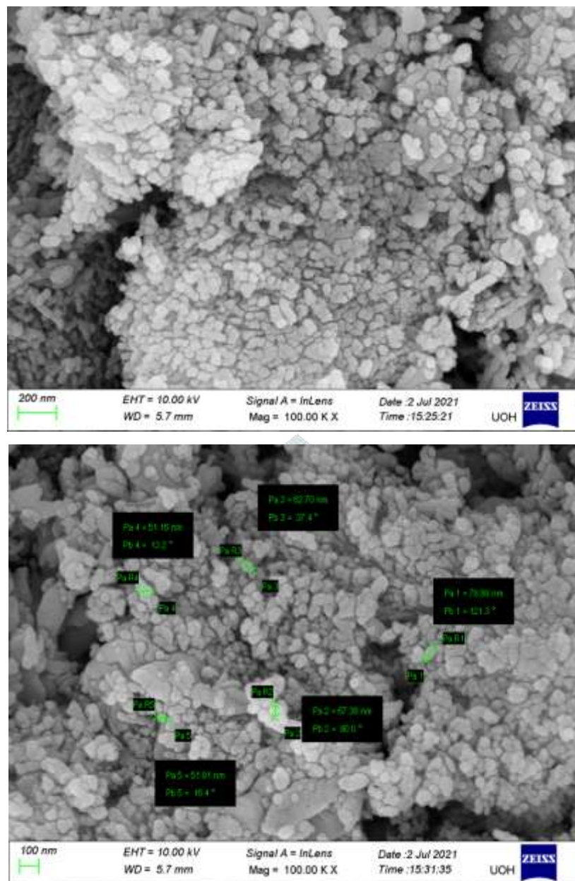
Figure 2: FESEM images of Gd-Nd co-doped \text{CaWO}_4 nano-crystals
