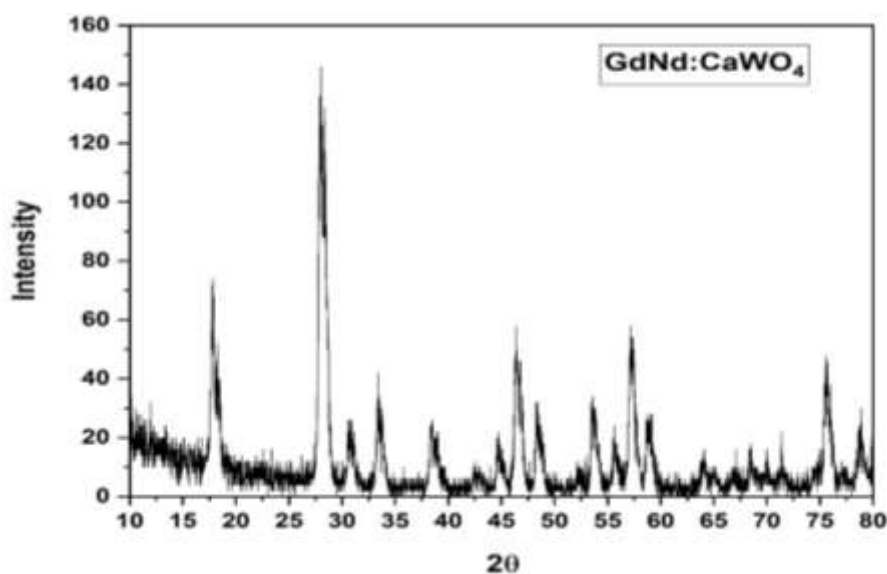
Figure 1: XRD pattern of the sample, confirming the formation of pure \text{CaWO}_4 phase.
