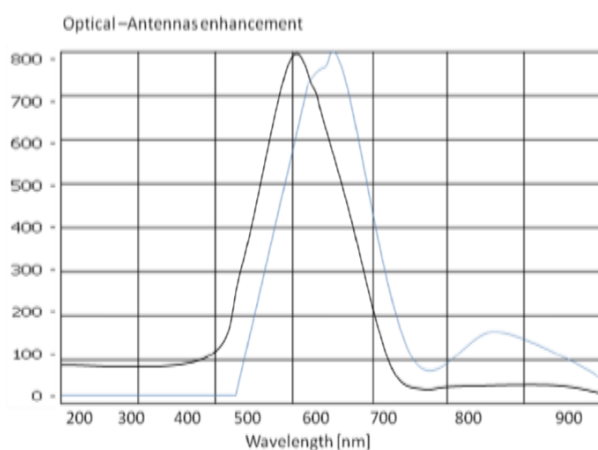
Fig.1.3.Optical DRA -Enhancement
