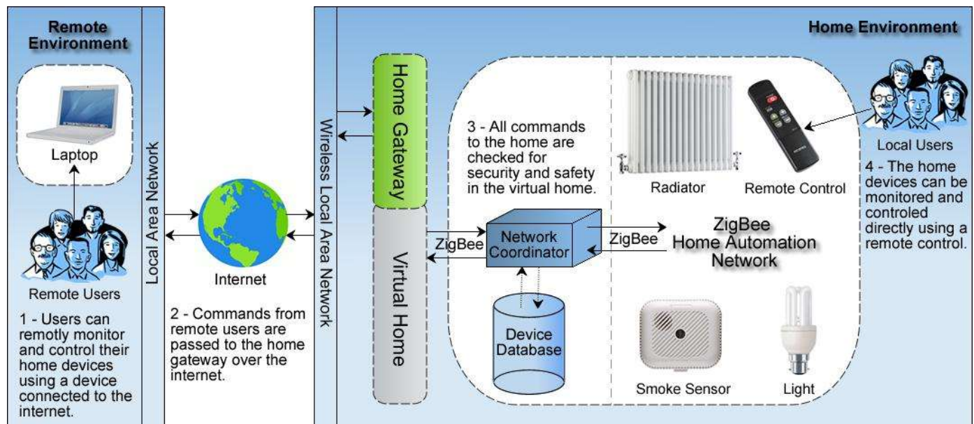
Fig. 1. Conceptual Architecture Overview
