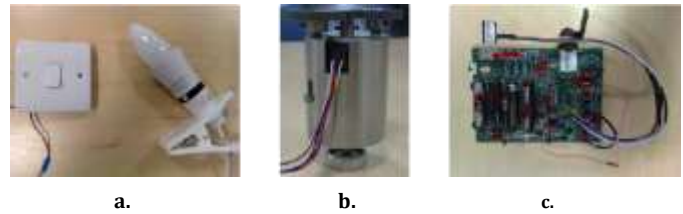
Fig. 6. (a) ZigBee operated light bulb in the off state; (b) ZigBee based automatic radiator valve; (c) ZigBee safety sensor.
