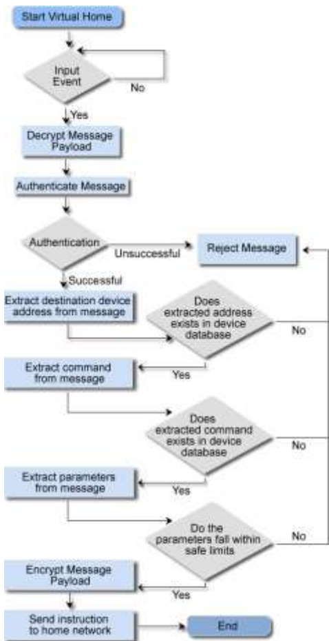
Fig. 5. Virtual Home Flow Chart.
