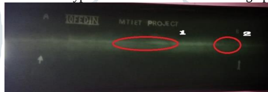
Fig 7.1: Radiographic film of Existing Parameters
