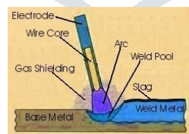
Fig4.1 SMAW welding Process
