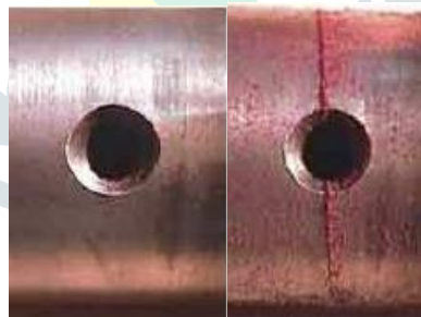
Fig5.4 workpiece performing magnetic particle testing
