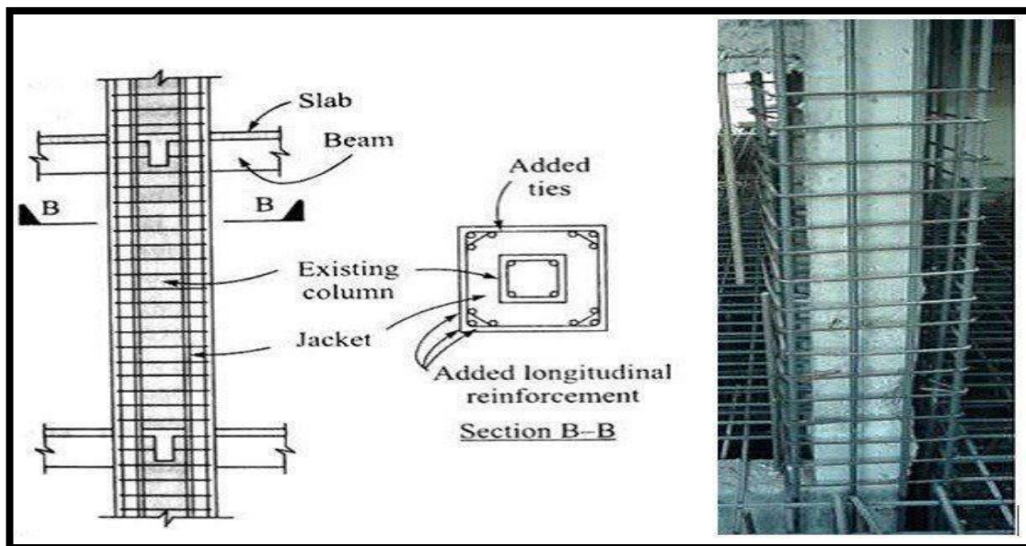
Fig. 1. Column Jacketing
