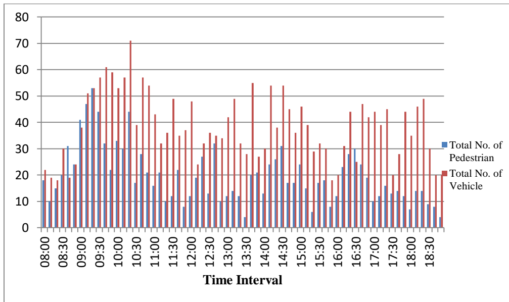
Figure 4: L-turn 02 of Sanatnagar Bypass intersection (Chanapora to Rawalpura)
