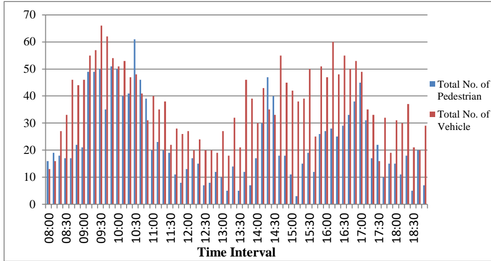
Figure 3: L-turn 01 of Sanatnagar Bypass Intersection (Baghat to Chanapora)
