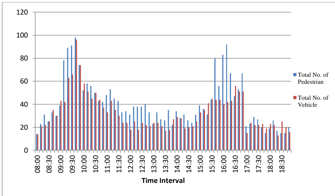
Figure 9: L-Turn03 of Hyderpora Bypass Intersection (Sanat Nagar to Airport)
