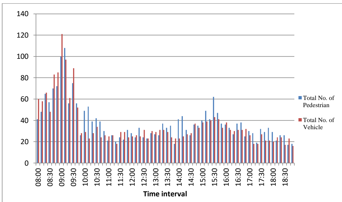
Figure 10: L-Turn 04 of Hyderpora Bypass Intersection (Airport to Tengpora)
