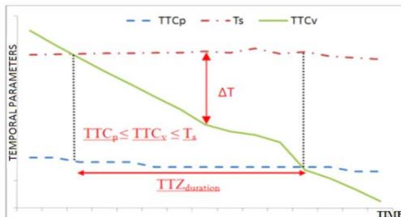
Figure 2: Showing Potential Conflict Time ( TTZ_{duration} )
