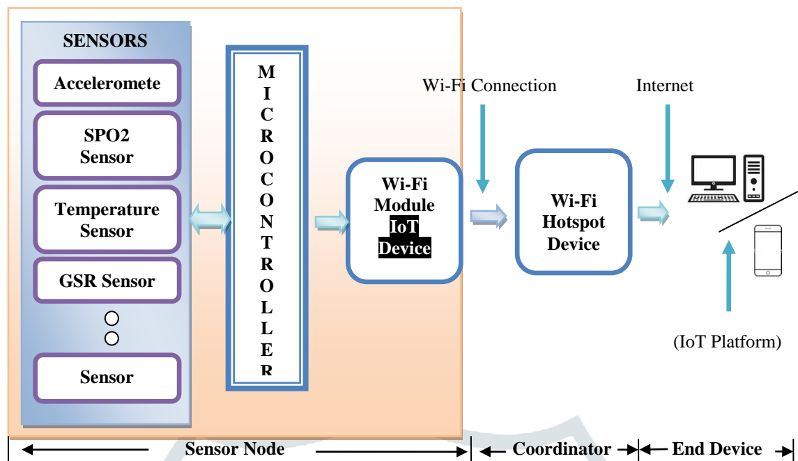
Figure 2: Functional block diagram of the system
