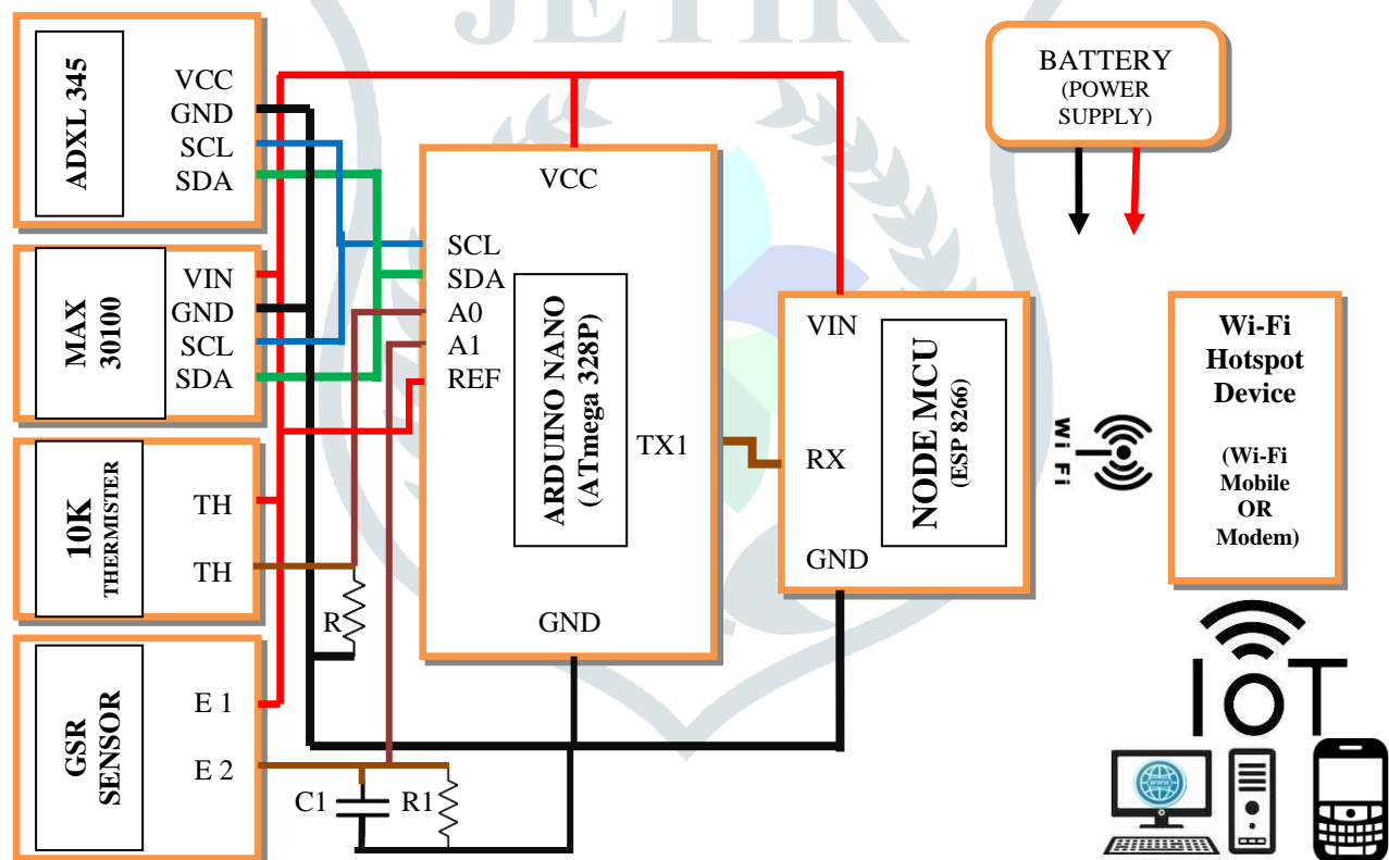
ig.4: Configuration of the system (Circuit Configuration of Sensor Node)
