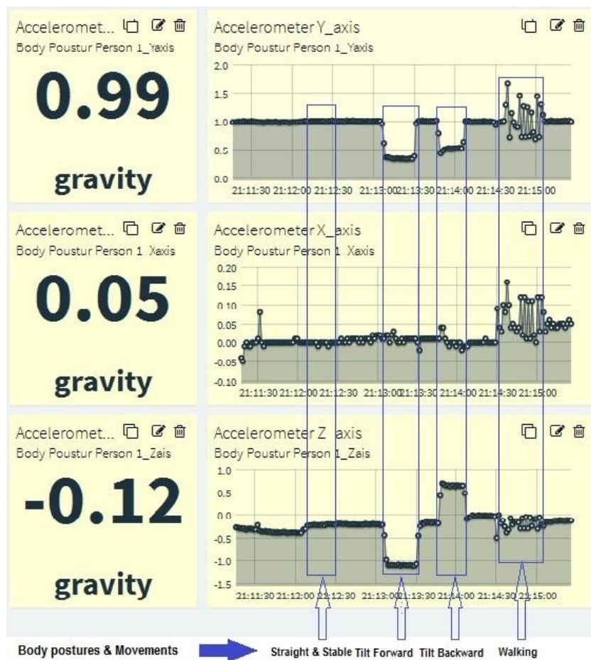
Fig.7: Widget for various parameters of sensor node 1(Person 1)
