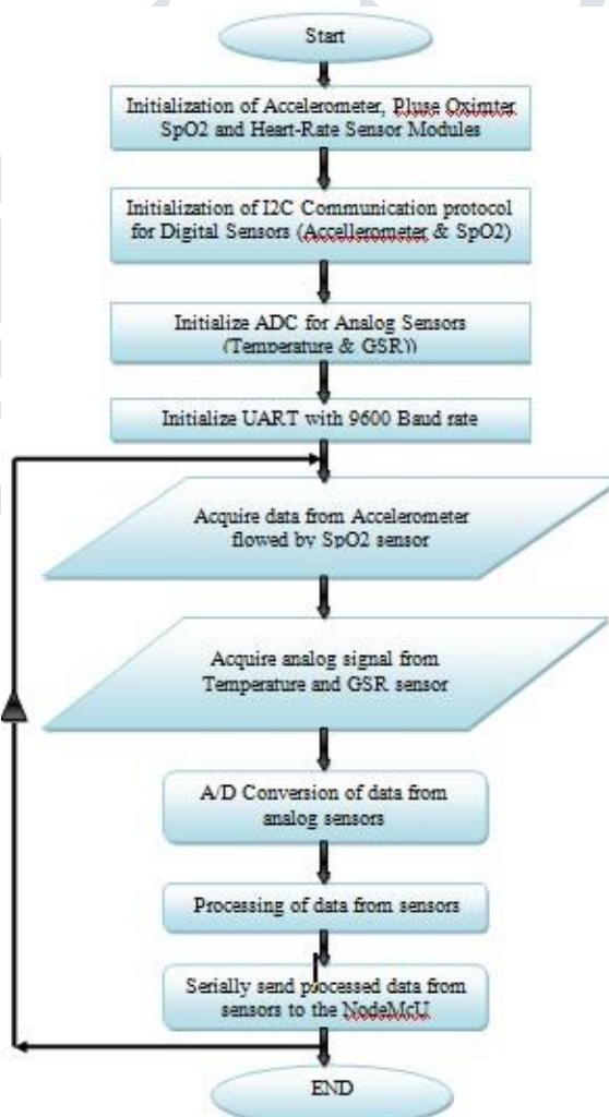
Fig. 6: Program Flow chart for Arduino Nano (µC-ATmega328)
