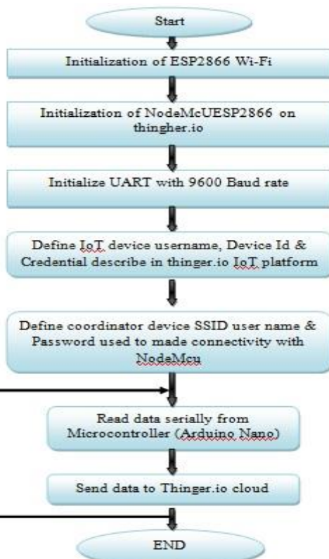
Fig. 5: Program Flow chart for NodeMCU Wi-Fi board
