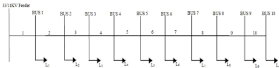
Fig.2. Standard 10 Bus RDS for Reliability studies
