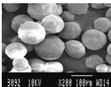
Figure 6: SEM of Foptima 1
