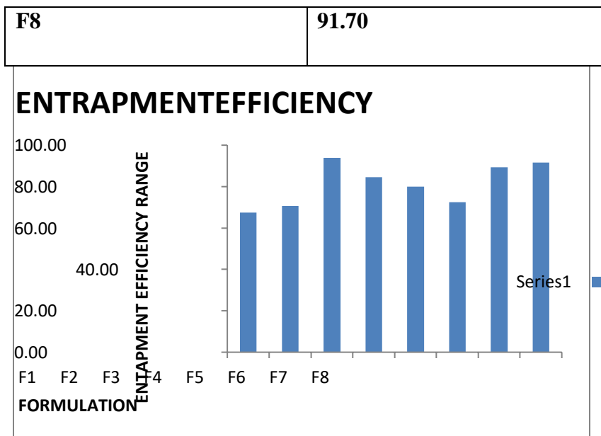
Figure 8: Entrapment Efficiency
